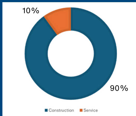
Operations Structure
